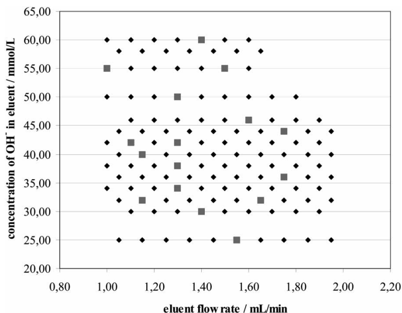
Figure 2. Design of 128 experimental data points: concentration of \text{OH}^- in eluent vs. eluent flow rate. The 16 experimental data points used for retention modeling are marked.
